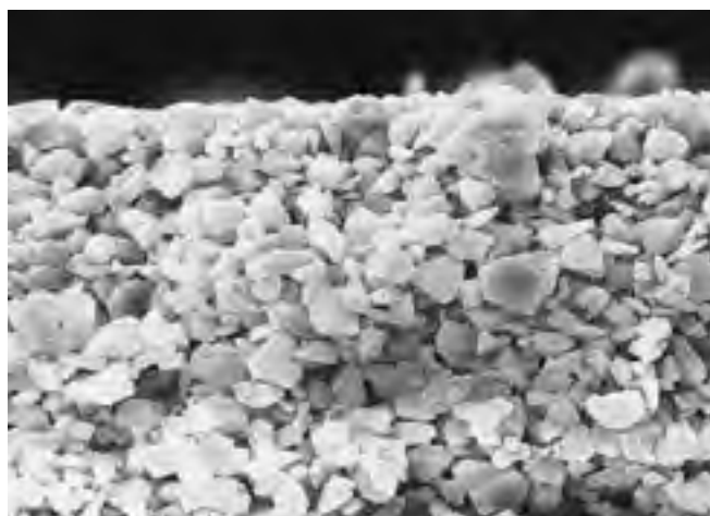
Electron microscope photograph of a cross section through an aluminum sheet with silica layer (magnification \times 500 )
